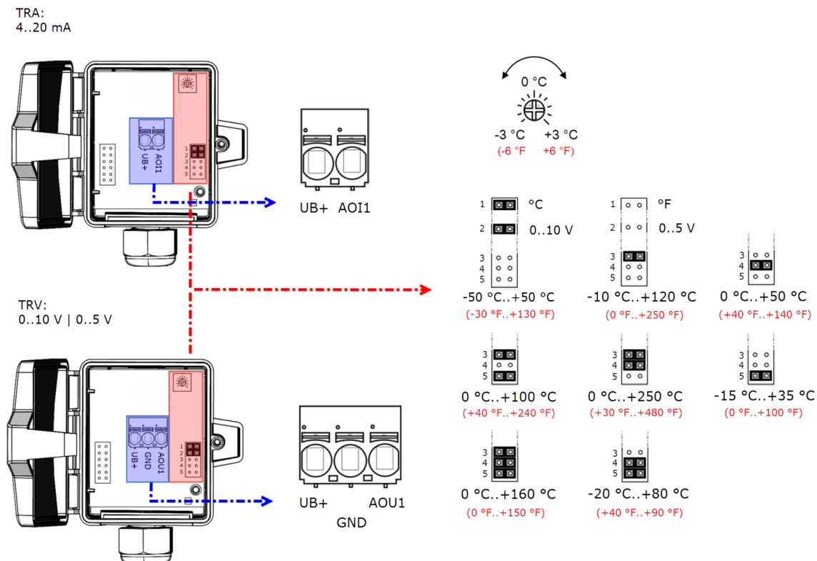
fig. (Measuring range and offset adjustment, default settings: -20 °C..+80 °C | 0 K)
